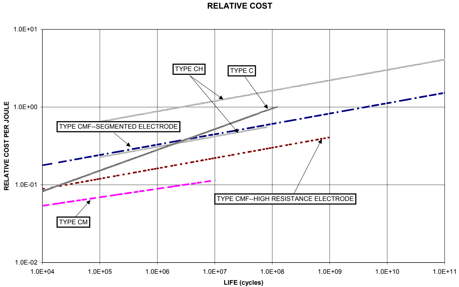
Figure 2. Relative Cost Per Joule versus Life of different high energy capacitor technologies.
