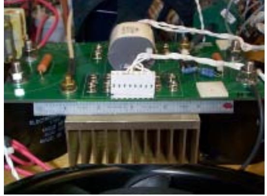
(a) Photograph showing a power stage with 3-layer printed circuit.
