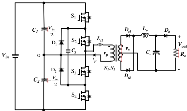
Figure 1. ZVS 3-level dc-dc converter for dc power supplies.
