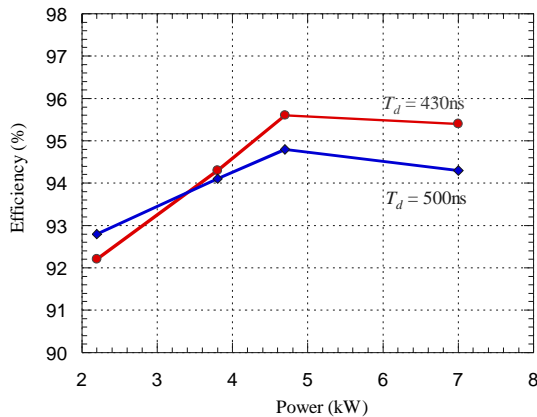
Figure 7. Efficiencies of the converter under different loads.
