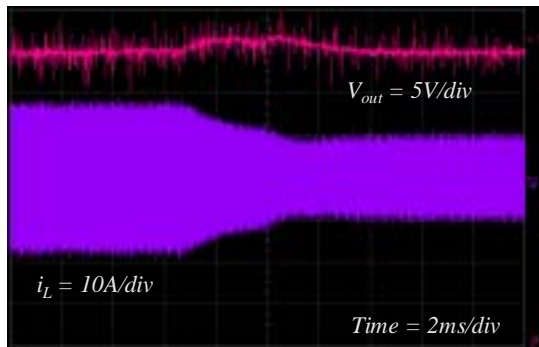
(a) Load change from 100% to 50%
