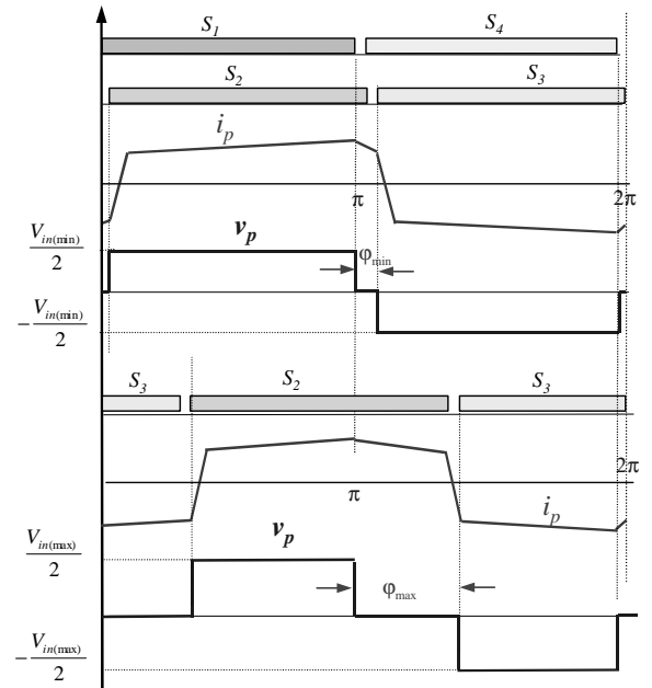
Figure 2. Voltage and current waveforms of the converter.
