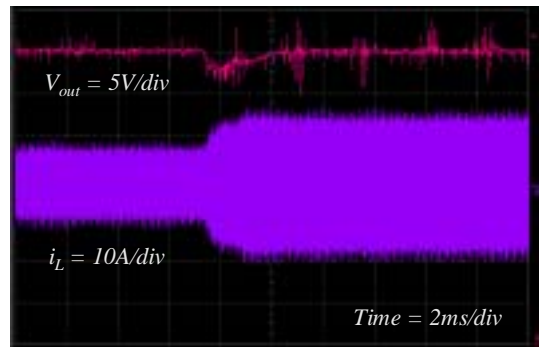
(b) Load change from 50% to 100%
